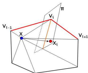
Figure 3. Illustration of the angle-based quality improvement algorithm.
