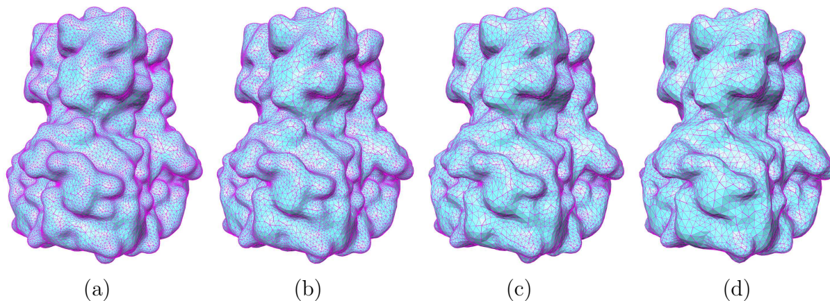
Figure 11. Multilevel mesh generation by coarsening (experiments on 1BVP). The parameter T_0 is described in Equation (6). The original mesh has 150,182 nodes and 300,360 triangles and is coarsened for two iterations with different coarsening parameters T_0 . (a) T_0 = 0.1 . Nodes = 26,842, Triangles = 53,680. (b) T_0 = 0.3 . Nodes = 19,588, Triangles = 39,172. (c) T_0 = 0.5 . Nodes = 12,882, Triangles = 25,760. (d) T_0 = 0.7 . Nodes = 9,480, Triangles = 18,956.
