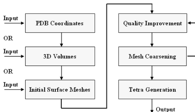
Figure 1. Illustration of our mesh generation toolchain. The inputs can be a list of atoms (with centers and radii), a 3D scalar volume, or a user-defined surface mesh. The latter two can be thought of as special cases of the first one.
