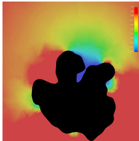
Figure 12. ACh distribution around the mAChE enzyme at the steady-state diffusion stage simulated by the SMOL solver [17]. Red corresponds to ACh concentration in the bulk, blue to a concentration of zero.
