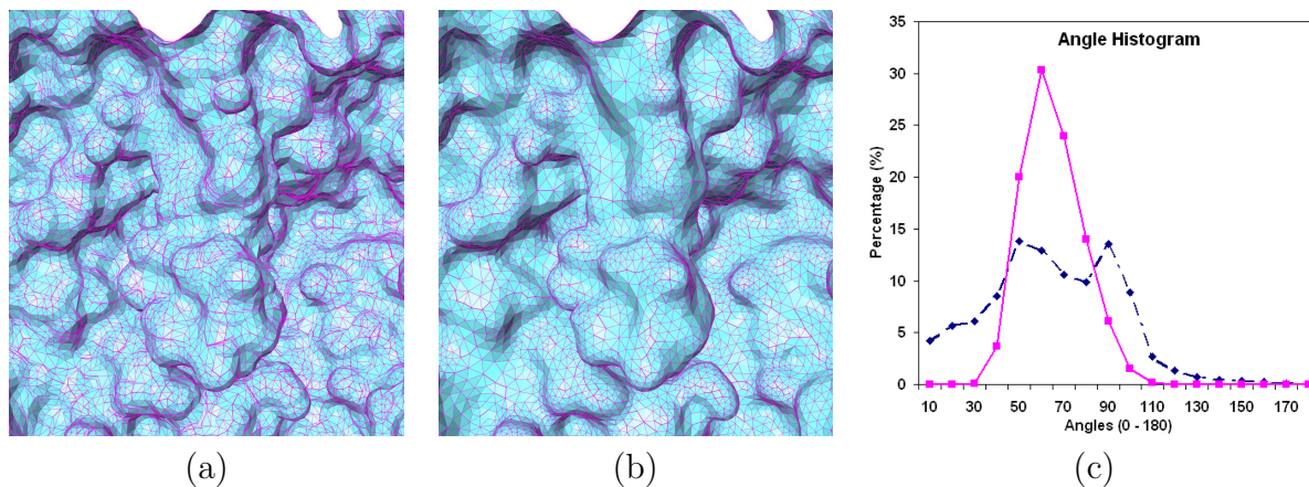
Figure 10. Mesh quality improvement on a user-specified surface mesh. (a) Original mesh generated by MSMS. (b) After mesh coarsening and quality improvement, the mesh size is about half as large as the original one, and the quality becomes significantly better. (c) The angle distributions of the meshes before (dashed or black line) and after (solid or purple line) the mesh post-processing.
