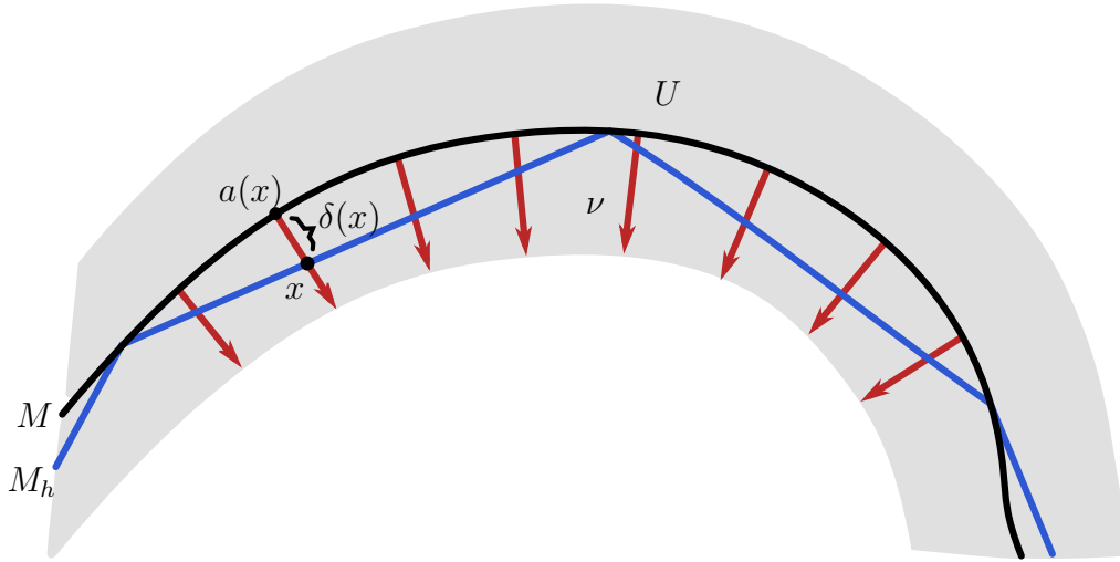
FIGURE 1. A curve M with a triangulation (blue polygonal curve M_h ) within a tubular neighborhood U of M . Some normal vectors \nu are drawn, in red; the distance function \delta is measured along this normal. The intersection x of the normal with M_h defines a mapping a from x to its base point a(x) \in M .
