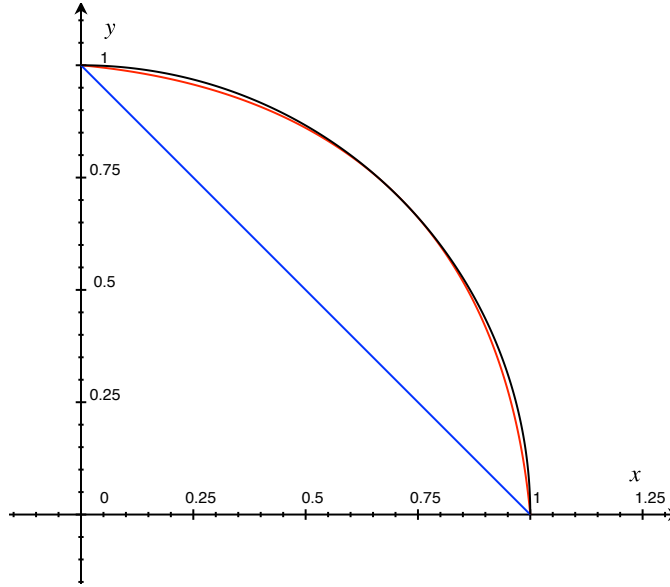
FIGURE 2. Approximation of a quarter unit circle (black) with a segment (blue) and much better quadratic Lagrange interpolation for the normal projection (red), though the underlying triangulation is the same (and thus also the mesh size).
