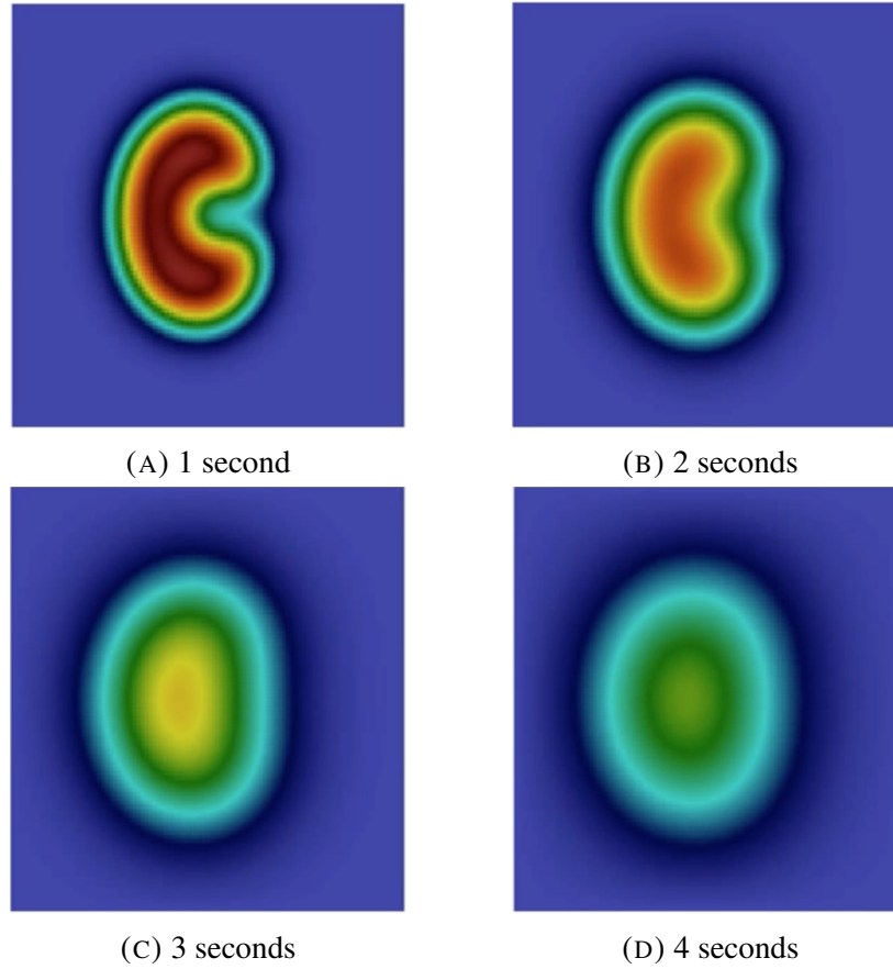
FIGURE 3. Hodge heat equation for k = 2 in a square modeled as a 100 \times 100 mesh, using the mixed finite element method given above. Initial data is given as the (discontinuous) characteristic function of a C-shaped set in the square. The timestepping method is given by the backward Euler discretization, with timestep \Delta t = 5 \times 10^{-5} .
